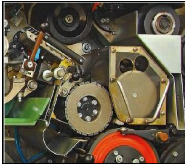
Shear Cut Unit
